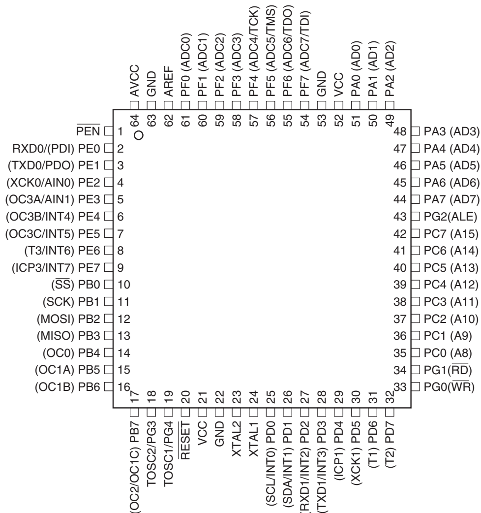
Figure 1. Pinout ATmega128
